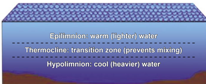
Figure 7. Lake Stratification.
