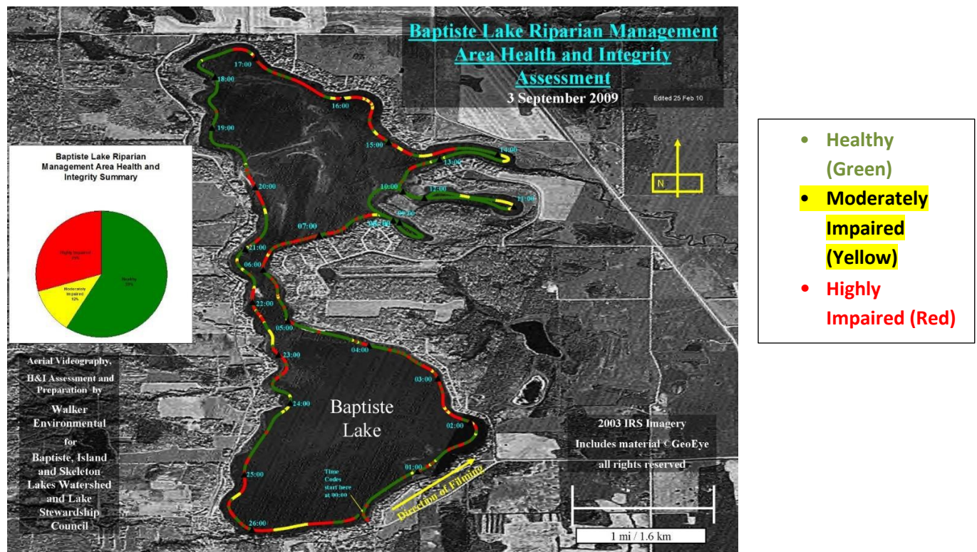
Figure 11. Riparian health rankings for the shoreline of Baptiste Lake in 2009.
